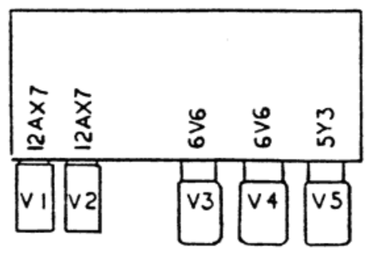
TUBE PLACEMENT
